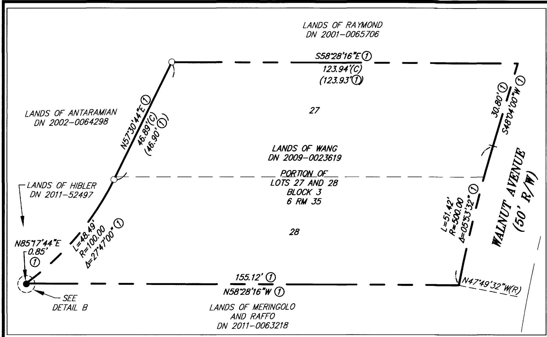
DETAIL A
